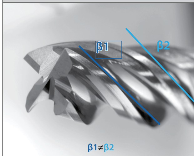
Variable Lead of Peripheral Cutting Edge
