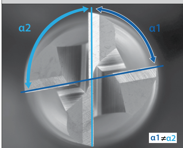
Unequal Spacing of End Teeth
